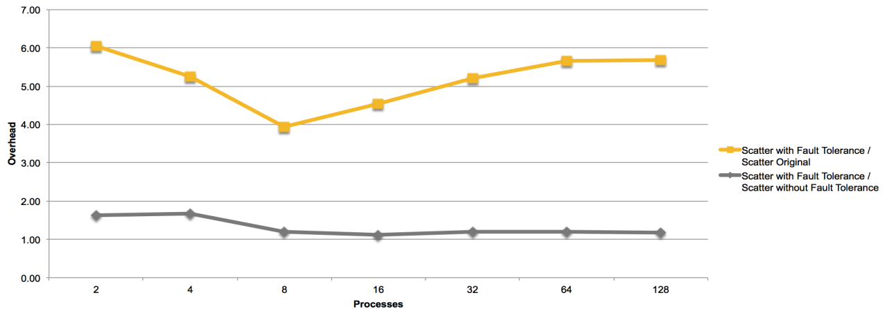
Figure 5.7: Scatter Overhead
