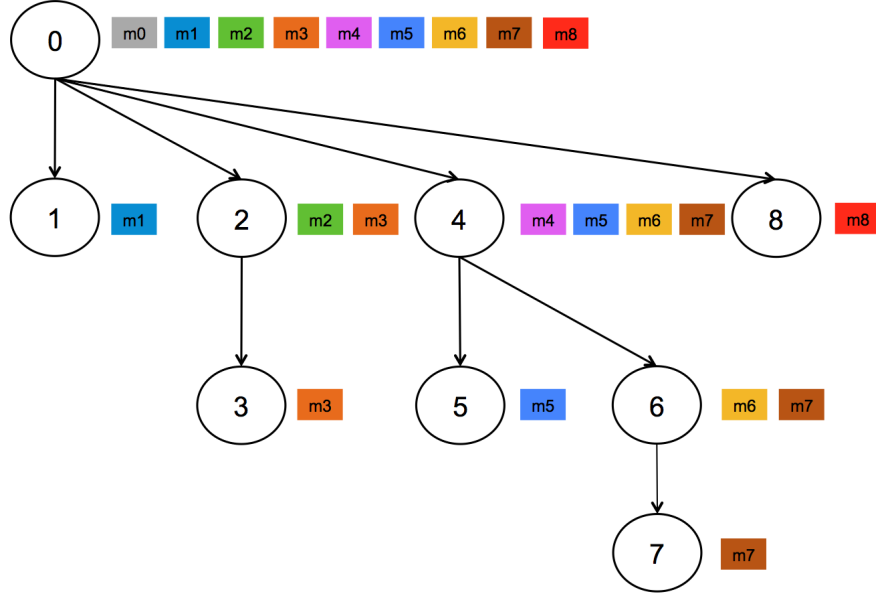
Figure 3.4: Binomial Tree Scatter
