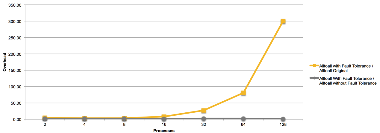
Figure 5.13: All-to-all Overhead
