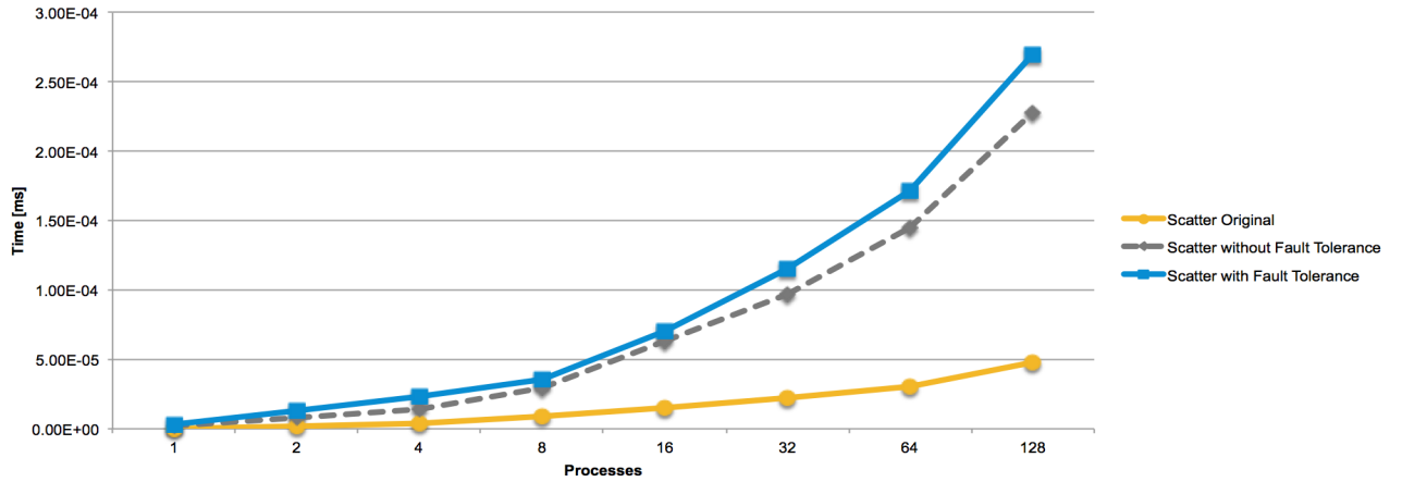
Figure 5.6: Scatter Runtime
