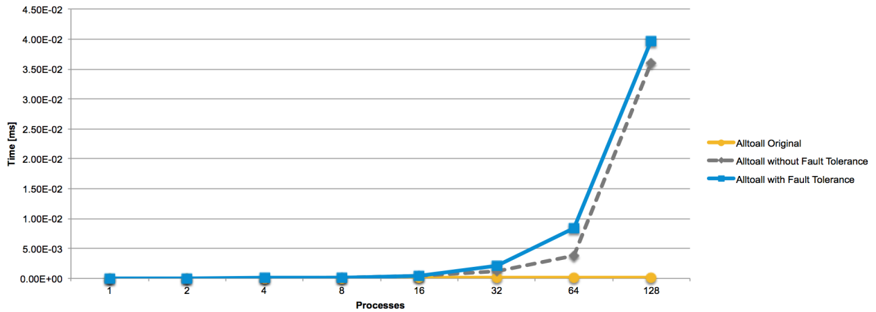
Figure 5.12: All-to-all Runtime
