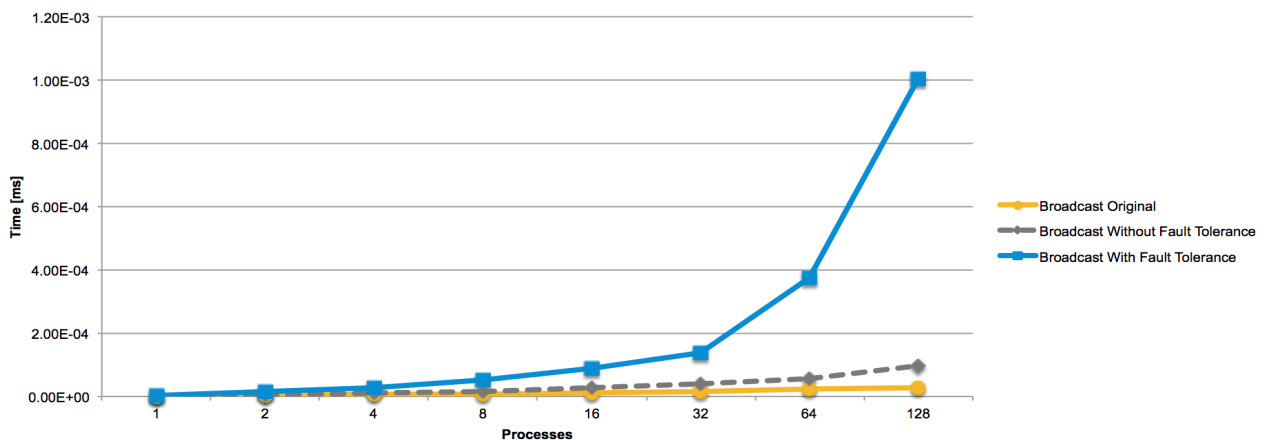
Figure 5.3: Broadcast Runtime
