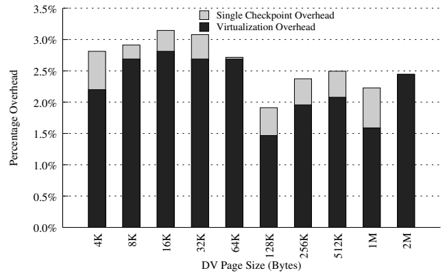
Figure 4. Comparison of DejaVu overhead for Sander vs. normal execution without DejaVu
