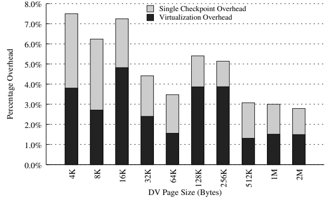
Figure 3. Comparison of DejaVu overhead for Chombo vs. normal execution without DejaVu
