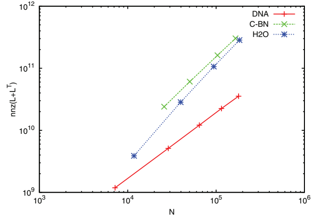
Figure 4. Number of non-zeros in the Cholesky factor of H for the systems shown on figure 5, as a function of the dimension of H .
