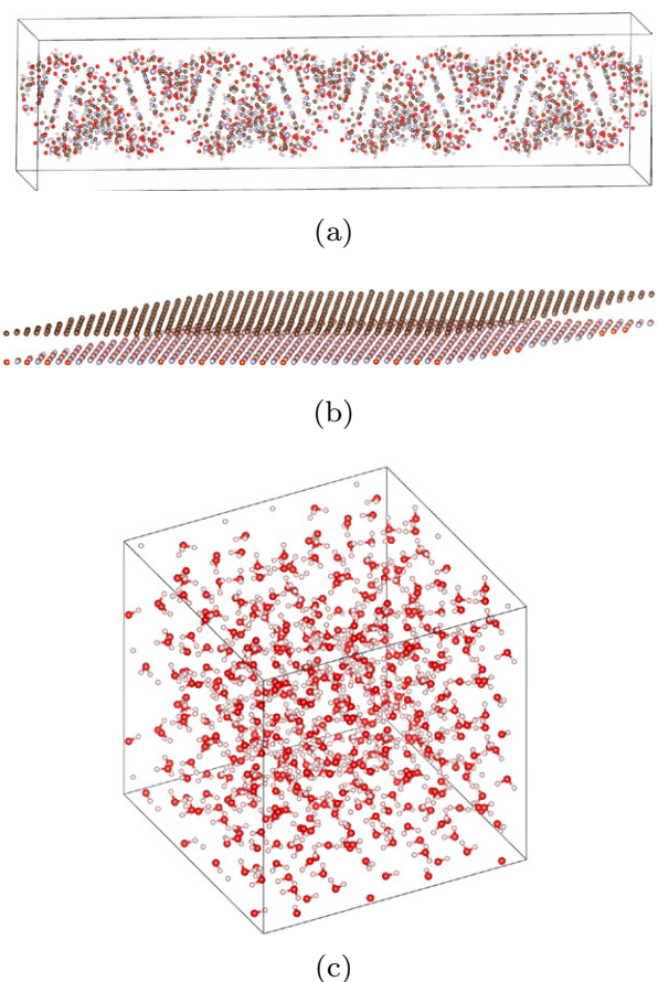
Figure 2. The atomic configuration of (a) the DNA-4 system (b) the C-BN 2,3 system and (c) the H 2 O-8 system.
